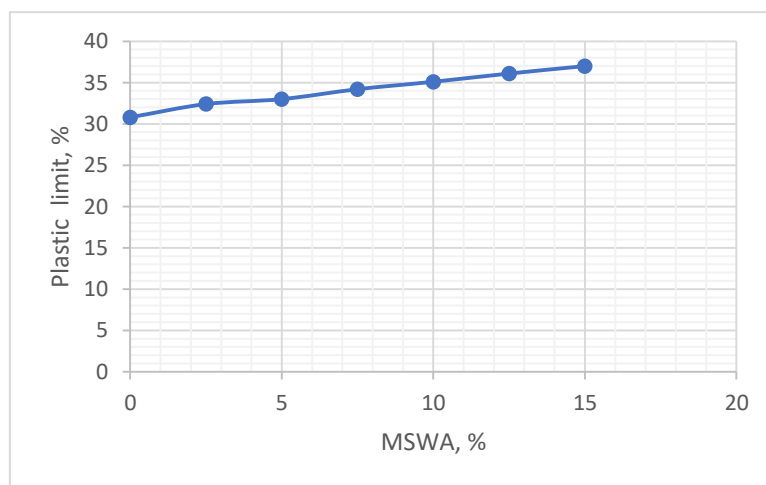
Fig. 2: Plastic limit test results.
