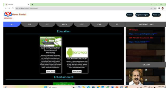
Fig. 2: Home Page
