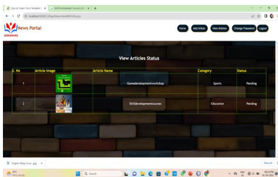
Fig. 4: View Articles
