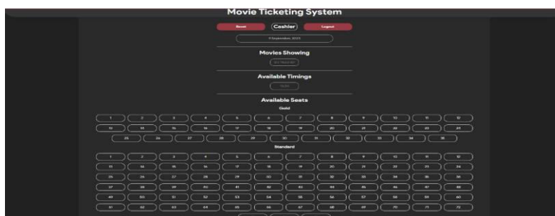
FIG 3 AVAILABLE SEATS
