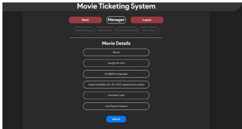
FIG 2 MOVIE DETAILS
