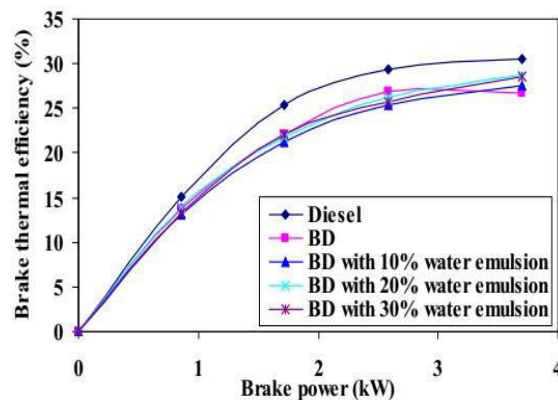
Fig. 2. Variations of brake thermal efficiency with BP
