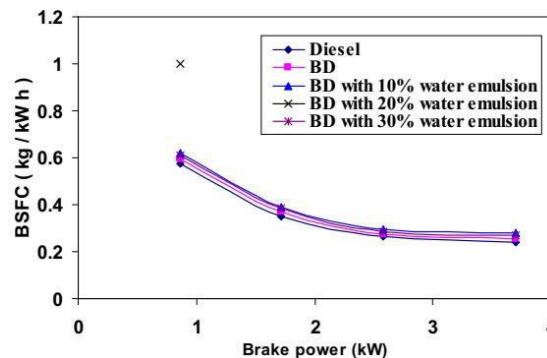
Fig. 3. Variations of brake specific fuel consumption with BP
