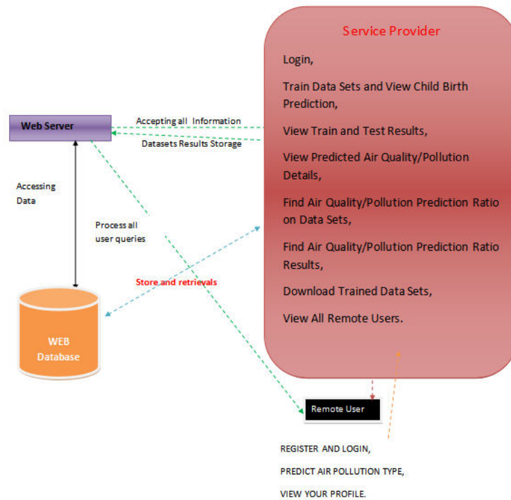
Fig1: System Architecture
