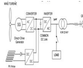
Fig. Hybrid PV-wind system connected to grid
