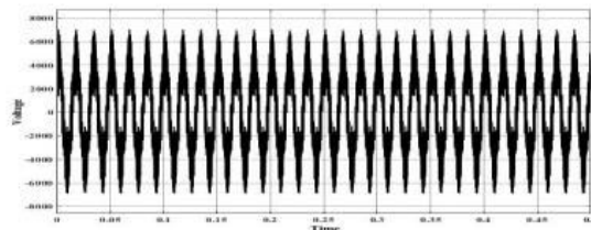
Fig.12 Photo Voltaic (PV) output voltage in hybrid system (per unit)
