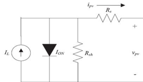
Fig.3.2 Equivalent circuit diagram of the PV cell
