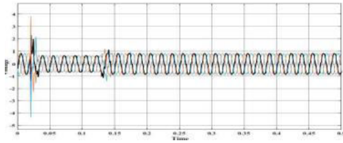
Fig.10 Wind turbine output voltage in hybrid system (per unit)
