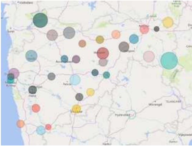
Fig 3 - Indicators for the rate of child mortality in various districts of Maharashtra where the size of the indicators is directly proportional to the extent of mortality in that particular district.
