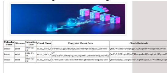
Figure 7: Confirmation Page
