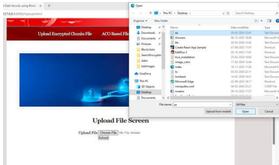
Figure 6: File Upload
